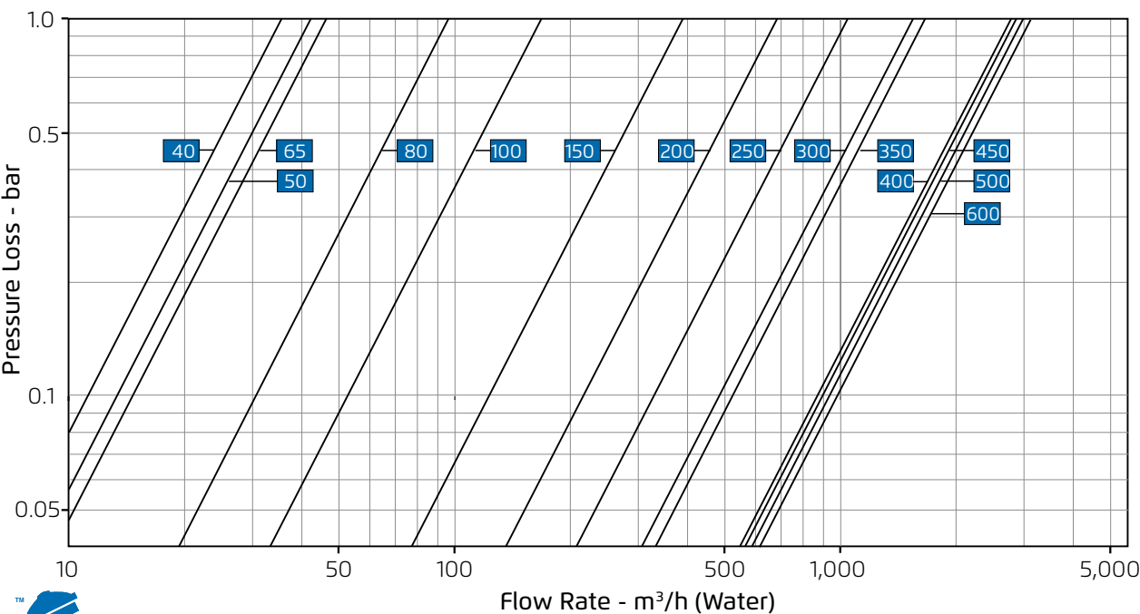
700 Y Pattern, Throttling Plug (V-Port)
